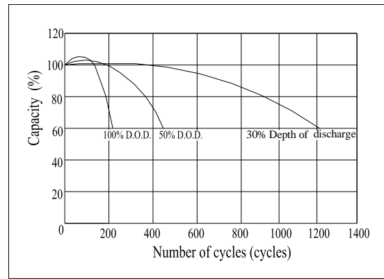
Cycle Life(25°C)
