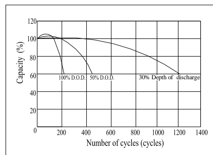
Cycle Life(25°C)
