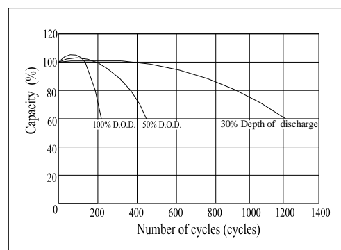
Cycle Life(25°C)
