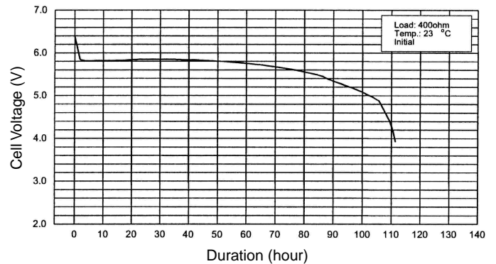
Discharge Characteristics of 2CR5
